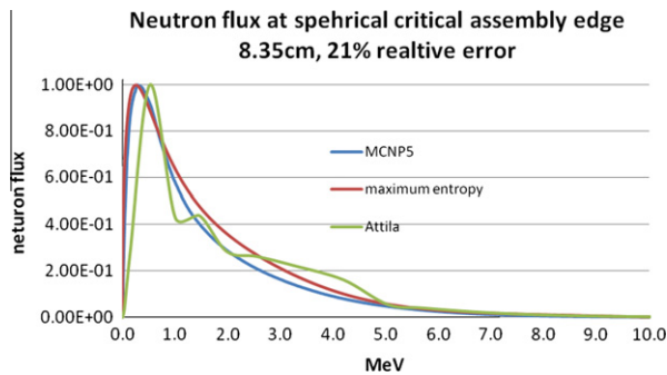
Fig. 2. Plot of the neutron spectrum for the three computation methods at the edge of the spherical critical assembly.
