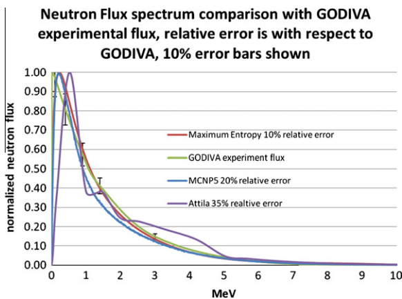
Fig. 3. Comparison plot of the three computational methods with the neutron spectrum from GODIVA, relative error is with respect to the GODIVA flux measurements.
