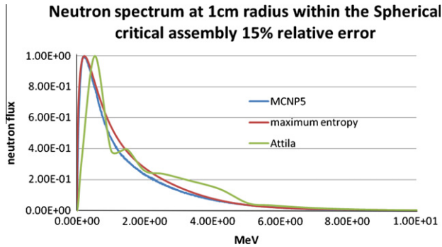
Fig. 1. Comparison plot of the three computational methods flux spectrum 1 cm radius within the spherical critical assembly.
